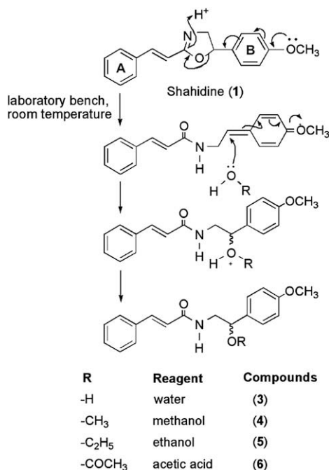
Scheme 2. Formation of amides (3–6) on addition of H 2 O, CH 3 OH, C 2 H 5 OH, and CH 3 COOH, respectively, to compound (1).
