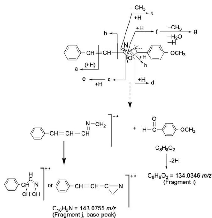
Scheme 1. Mass fragmentation of shahidine ( 1 ).
