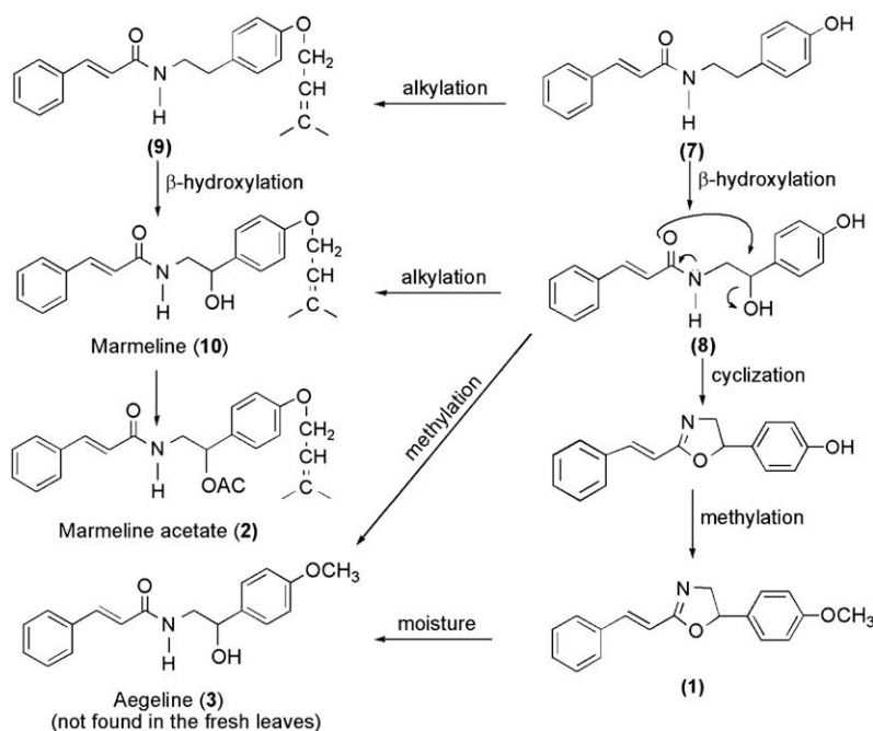
Scheme 3. Proposed biogenetic pathway for the formation of ( 1 ) and ( 2 ) in the fresh leaves of A. marmelos .
